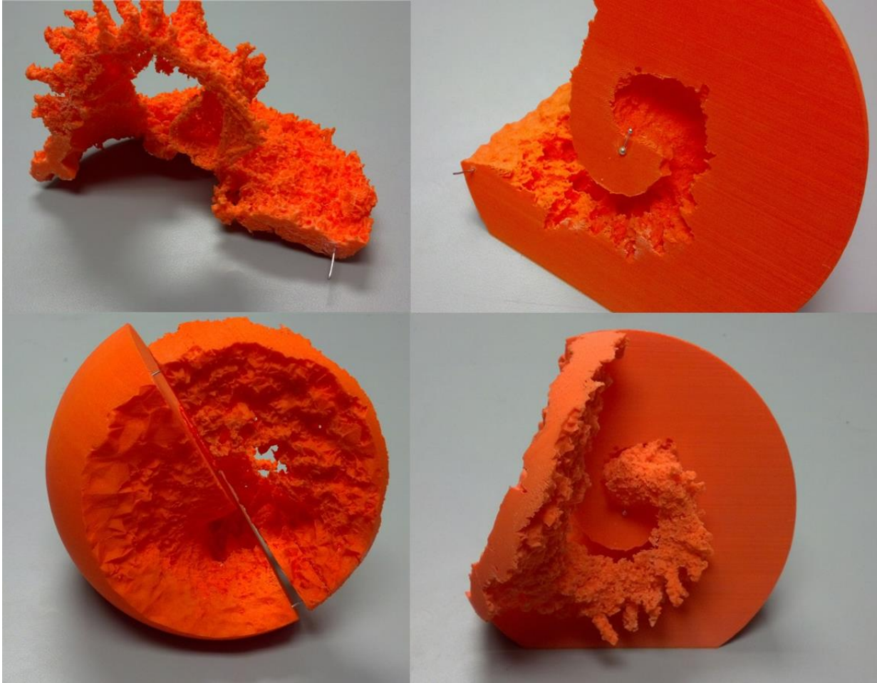
Figure 2. Example showing the placement of the metal pins used to connect the two component pieces of the 3D print model at orbital phase 1.045.
