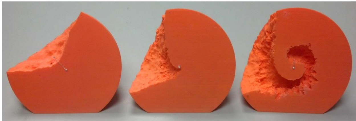
Figure 1. Example showing the beads representing the stars attached to each 3D print model listed in the above table. Orbital phases are, from left to right, apastron, periastron, and 1.045.
